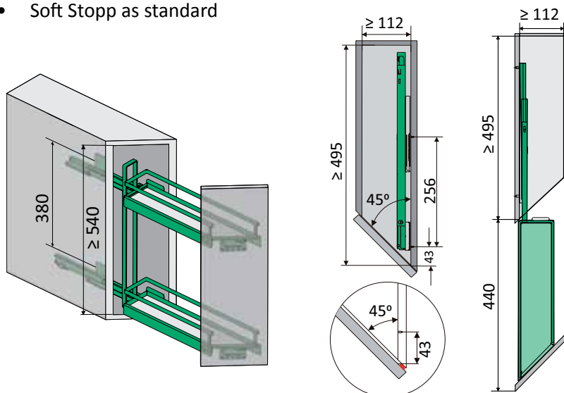
150 mm Angled Bottle Pull Out
