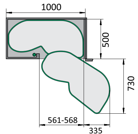
LeMans 600 Right Swivel
