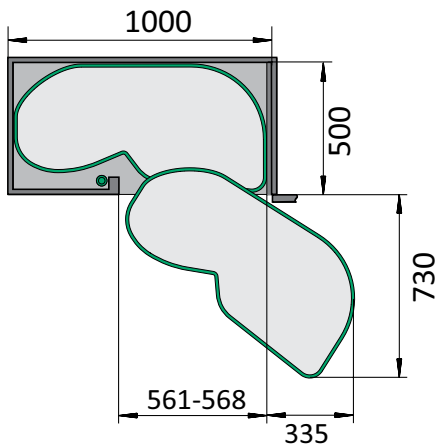
LeMans II - Order codes
