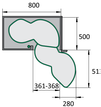
LeMans 400 Right Swivel
