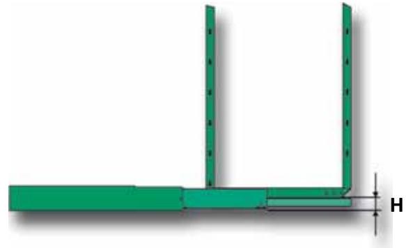
Dispensa Larder Runner - Technical
