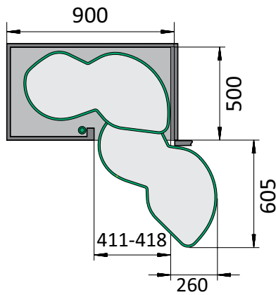
LeMans II 450 Right Swivel
