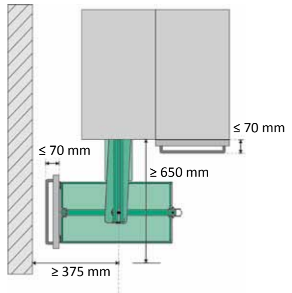
DISPENSA Swing Corner installation
