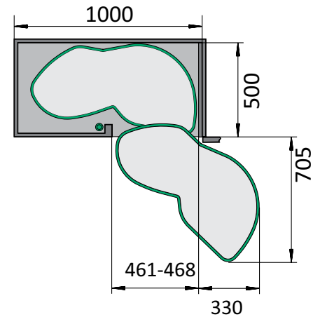
LeMans II 500 Right Swivel
