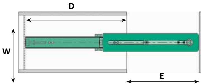
DISPENSA Swing - Dimensions
