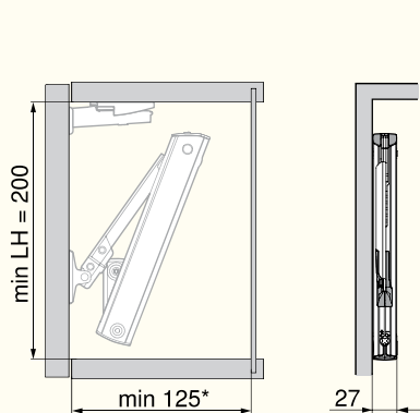
Space Requirement
