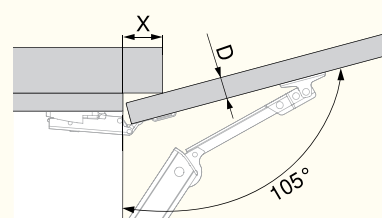
Cornice Clearance
