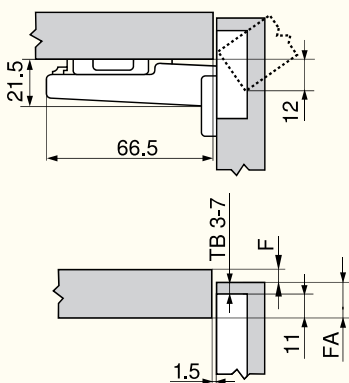
Hinge Positions
