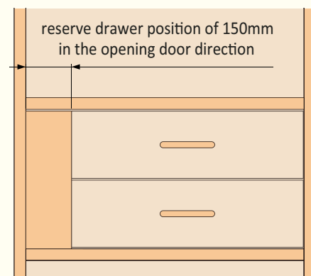
Minimum Gap
