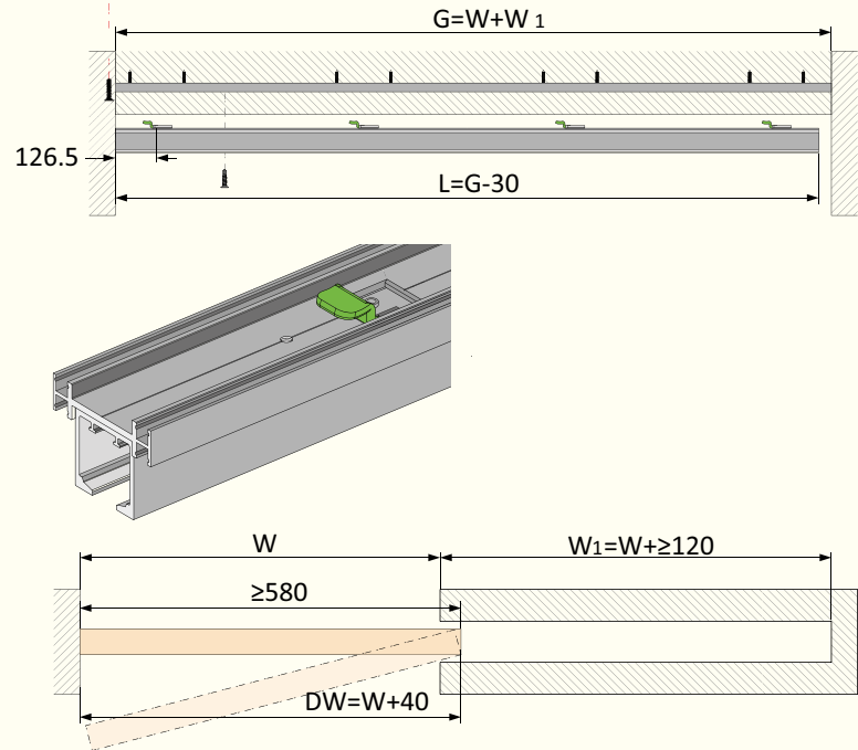
Track Dimensions
