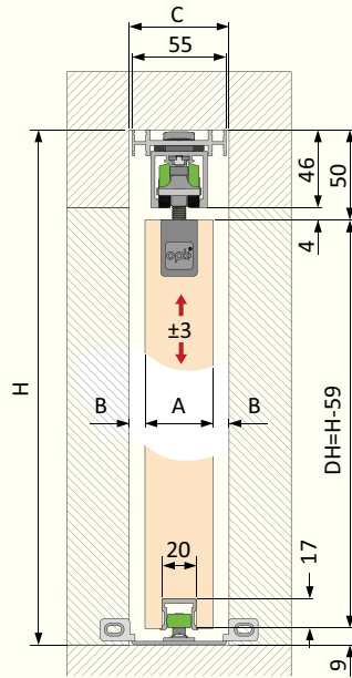
Pocket and Door Dimensions
