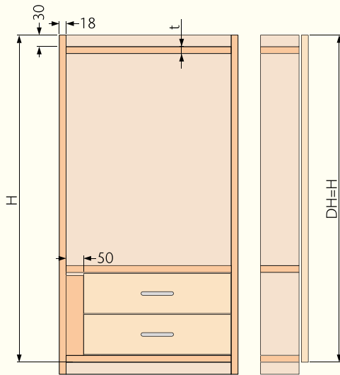
Outer Top Mounting
