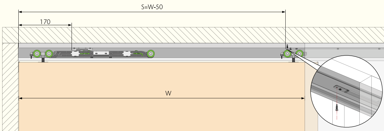
Fixing Positions
