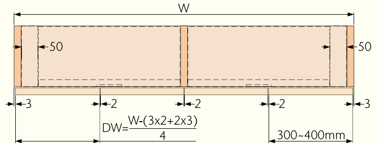
Four Doors
