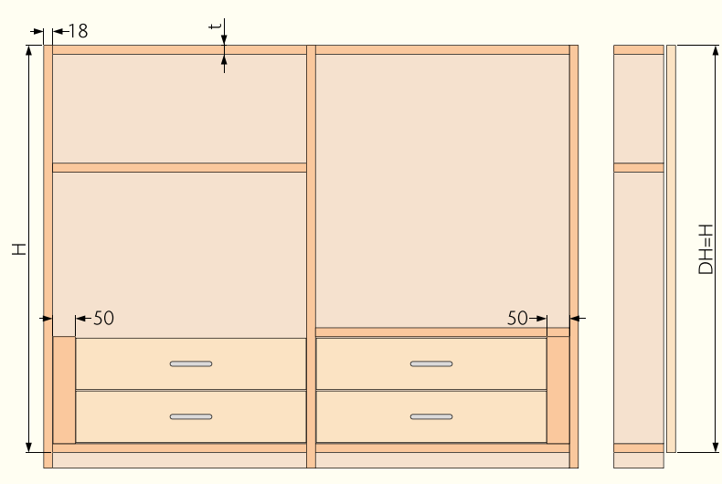
Inner Top Mounting
