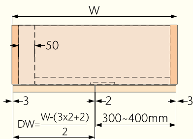
Two Doors
