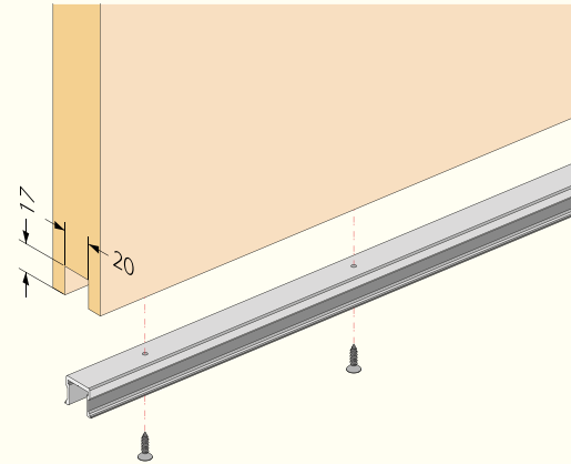
Fixing Positions
