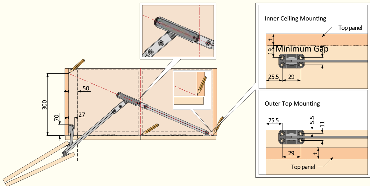
Pivot Arm fixing positions
